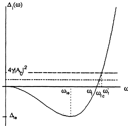
FIG. 7. Instability analysis using \Delta_I(\omega) for \beta_{2e} > 0 . The upper and lower dashed horizontal lines are 4\gamma|A_0|^2 and 2\gamma|A_0|^2 , respectively. The frequency range of instability corresponds to the section of \Delta_I(\omega) curve between horizontal axis and upper dashed horizontal line, i.e., (\omega_f, \omega'_f) . The intersection of the curve with the lower dashed horizontal line at \omega_{fc} indicates the frequency of maximum growth rate \gamma|A_0|^2 . As power increases, both horizontal lines go up.
