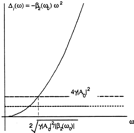
FIG. 1. Instability analysis using \Delta_I(\omega) = -\beta_2(\omega_0)\omega^2 . The upper dashed horizontal line is 4\gamma|A_0|^2 and the lower is 2\gamma|A_0|^2 . The frequency range of instability corresponds to the section of the \Delta_I(\omega) curve between the horizontal axis and upper dashed horizontal line. The intersections of the curve with the lower dashed horizontal line indicate the frequency of maximum growth rate \gamma|A_0|^2 . As power increases, both horizontal lines go up.
